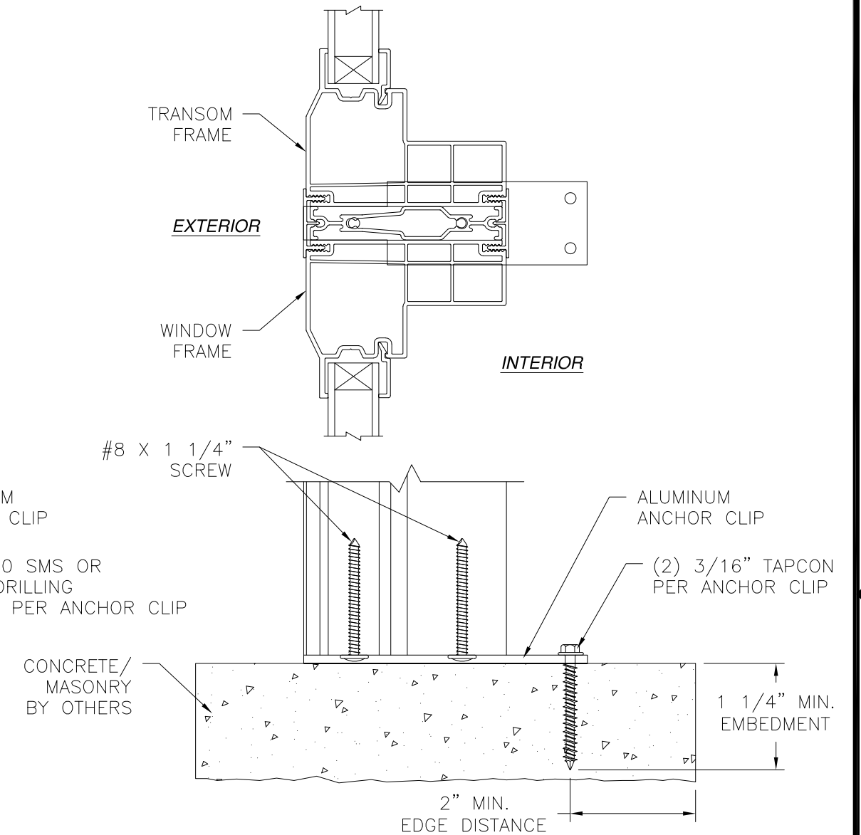
HORIZONTAL MULLION ANCHOR CLIP DETAIL CONCRETE/MASONRY INSTALLATION
